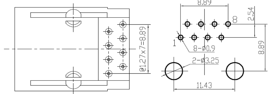
PC BOARD LAYOUT THICKNESS=1.6mm
