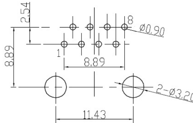
PC BOARD LAYOUT THICKNESS=1.60MM
