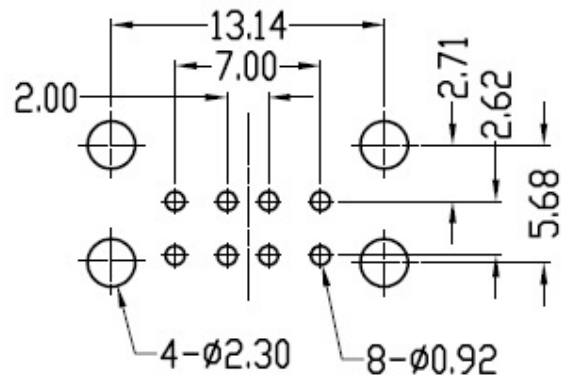
RECOMMENDED P.C.B HOLE LAYOUT TOP VIEW(TOLERANCE:±0.05)
