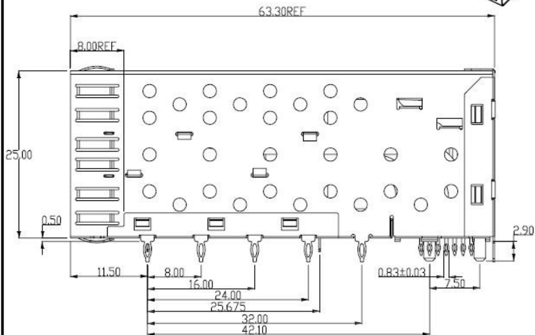
SFP 2x1 CAGE Assembly
