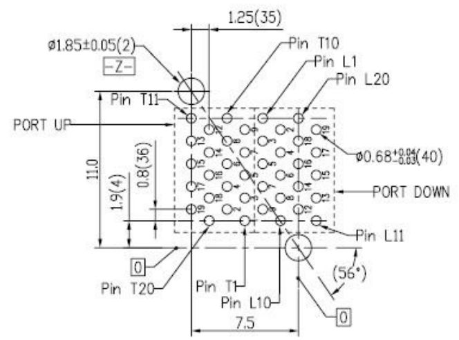
CONNECTOR PC Board Layout
